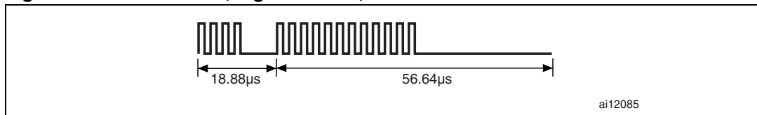
Figure 31. End of frame, high data rate, one subcarrier x2
