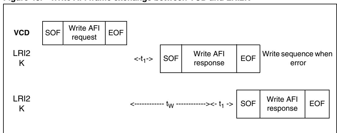
Figure 48. Write AFI frame exchange between VCD and LRI2K
